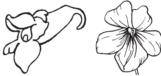
Irregular Flowers
