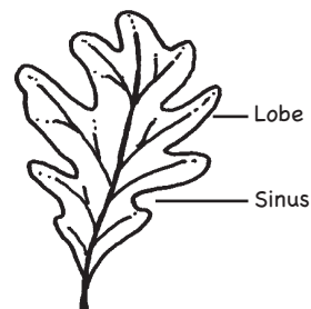
Lobed
