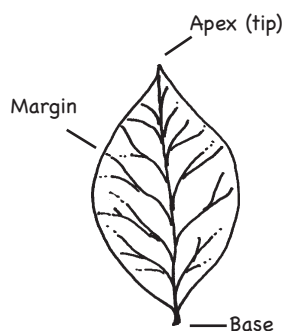
Entire (smooth)
