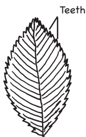
Toothed (serrated)
