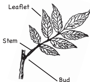
Pinnate
